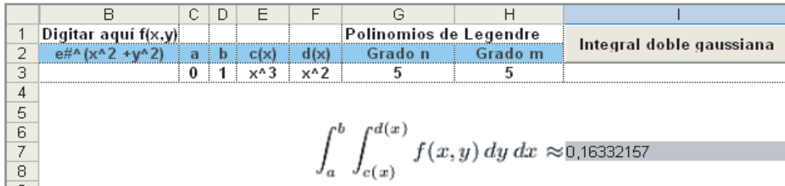
Figure 2.4: Integral doble gaussiana.
